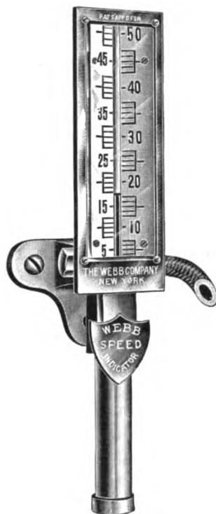
WEBB SPEED INDICATOR.
